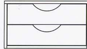
3782-502 WARDROBE SINGLE DRAWER INSERT inches: 25w 20d 13.5h centimeters: 63.5w 51d 34.5h 3782-503 WARDROBE DOUBLE DRAWER INSERT inches: 36w 20d 13.5h centimeters: 91.5w 51d 34.5h
