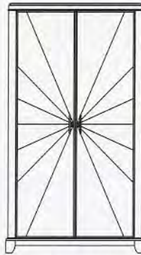
3563-501 DOUBLE WARDROBE inches: 41w 26d 76h centimeters: 104.5w 66.5d 193.5h
