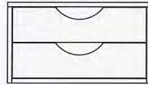
3563-502 WARDROBE SINGLE DRAWER INSERT inches: 25w 20d 13.5h centimeters: 63.5w 51d 34.5h 3563-503 WARDROBE DOUBLE DRAWER INSERT inches: 36w 20d 13.5h centimeters: 91.5w 71.5d 34.5h
